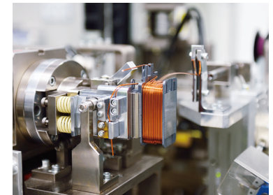
High-density coil winding machine for motors
