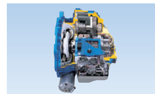
FWD 6-speed AT
