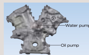
Timing chain cover integrated with water pump and oil pump
